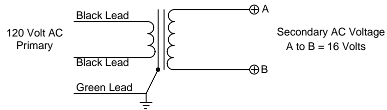
591 Transformer
